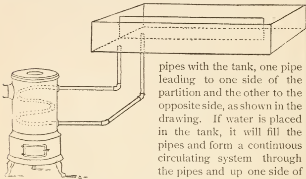
54. Barnard's propagating-tank.
